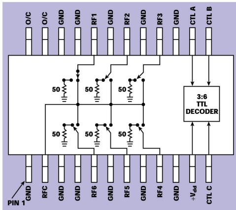
▲ Fig. 5 The HMC252QS24 SP6T functional diagram.
