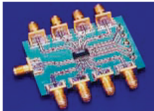
▲ Fig. 8 The HMC253QS24 SP8T switch evaluation PCB.
