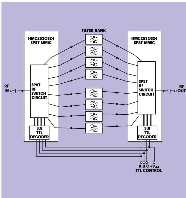
▲ Fig. 9 An eight-element switched filter bank utilizing two HMC253QS24 SP8T switches.
