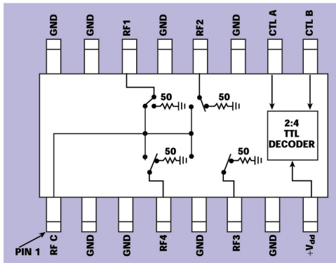
▼ Fig. 3 The HMC241QS16 SP4T functional diagram.
