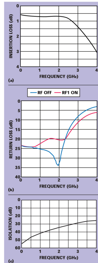
▲ Fig. 4 The HMC252QS24 SP6T switch's (a) insertion loss, (b) return loss and (c) isolation vs. frequency.
