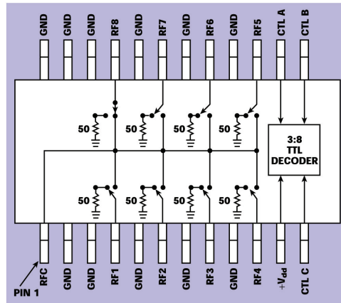
▲ Fig. 7 The HMC253QS24 SP8T functional diagram.
